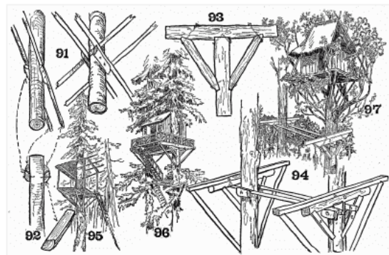
Details of tree-top houses.
