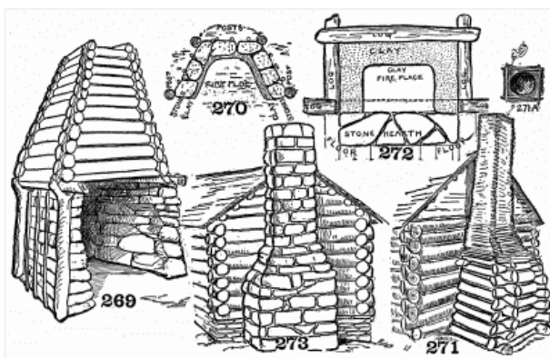
Detail for fireplaces and flues.
