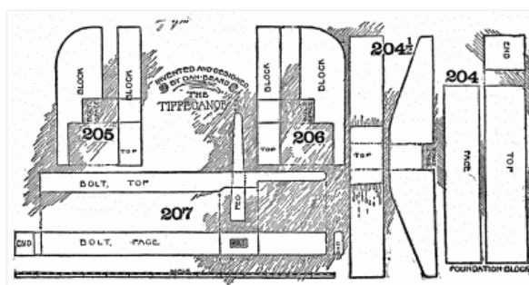
Detail parts of Tippecanoe door-latch.
